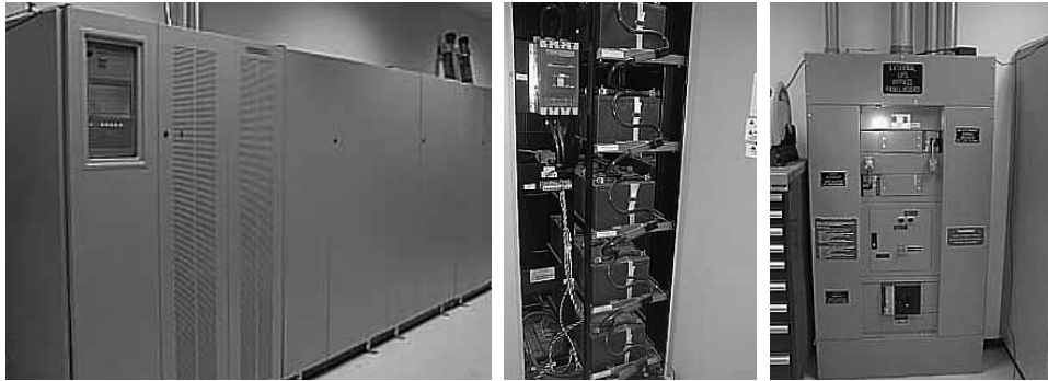
Figure 10.01: Typical UPS units (Source: Integral Group)
