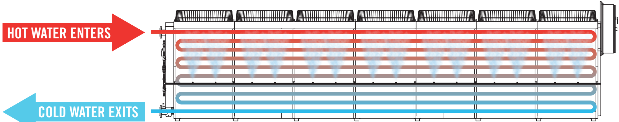
Cooling flow in a typical 7-fan VIRGA III ®
